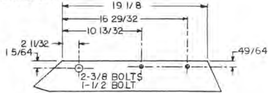
CA16-4RS CA16-4LRS
