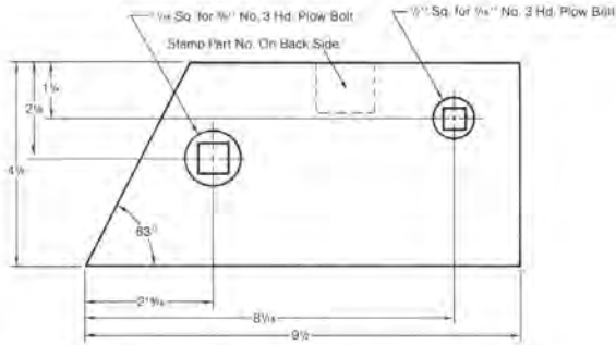
107981 Landside – FORD – Rear Landside 107981 R.H. Shown 108429 L.H. Opposite General Purpose Bottom
