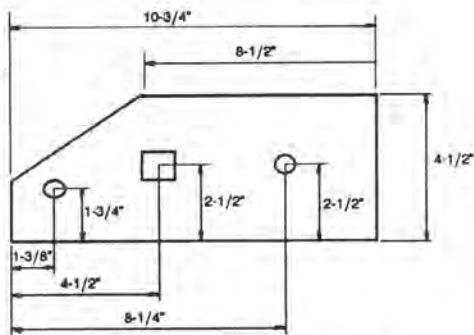
489465 RH LANDSIDE 542417 LH LANDSIDE 7/16 X 1-3/4 - 7/16 X 1-3/4
