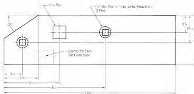
522343 Landside – IHC – “Rear” Landside Right Hand Shown Left Hand Opposite Super Chief Bottom
