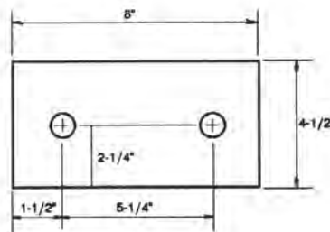
A27862 LANDSIDE 5/8 X 3-1/2-5/8 X 3-1/2
