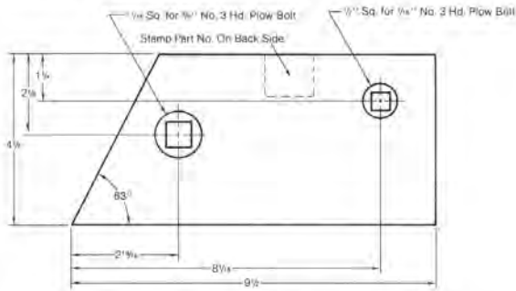
107981 Landside – FORD – Rear Landside 107981 R.H. Shown 108429 L.H. Opposite General Purpose Bottom
