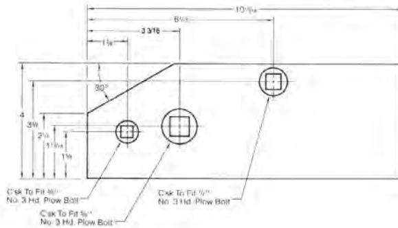
T10856 Landside – CASE PLOWS – Front or Rear Landside for EX Series Bottoms
