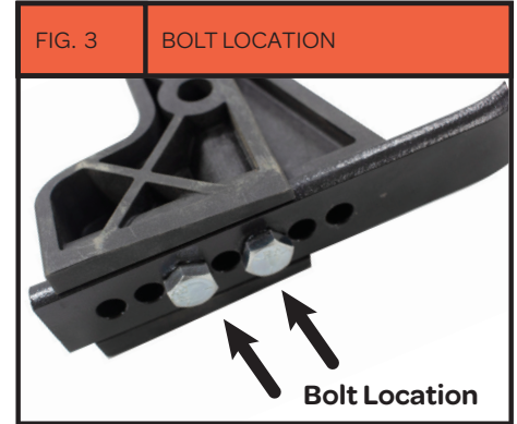
Fig3 Above highlights the bolt location for the Firmer block and the S Bar. Place the bolts in the 3rd and 5th hole openings. 1
