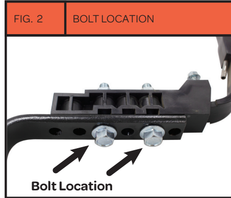
Fig 2 Above highlights the bolt location for the Firmer block and S Bar. Connect using 2 Standard Hex Bolts in the 3rd and 5th hole openings. 1
