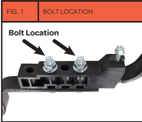
Fig. 1 Above highlights the bolt location for Firmer block. Connect using 2 Standard Hex Bolts in the 2nd and 4th hole openings. 1
