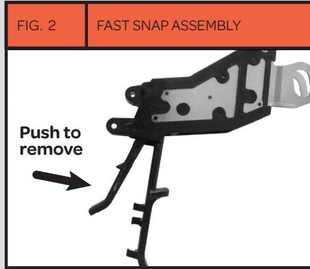
Fig 2 Above shows the tail inserted into the bracket. To remove the tail, press the tab on the tail. Pull down and remove from bracket.
