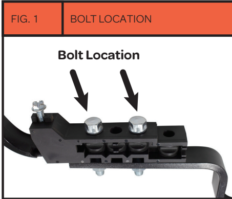
Fig. 1 Leave the first hole empty at the top of the firmer adapter and place the bolts in the 2nd and 4th openings. 1
