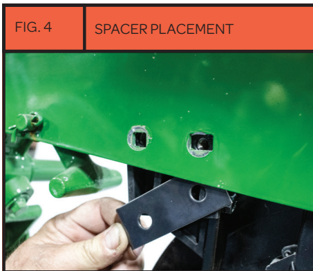
Fig. 4 Place the spacer in between the scraper holes and the firmer block like shown.
