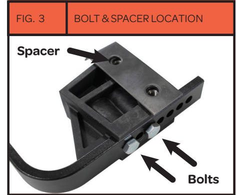
Fig 3 Above highlights the bolt location for Firmer block and S Bar. Place the bolts in the 1st and 3rd hole openings. 1
