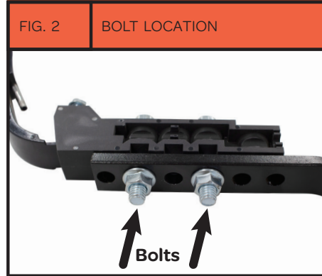
Fig 2 Above highlights the bolt location for Firmer block and S Bar. Connect using 2 Standard Hex Bolts in the 2nd and 4th hole openings. 1
