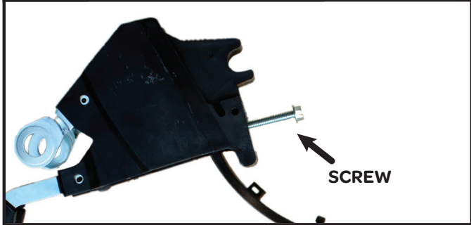
FIG. 2 TIGHTEN SCREW
