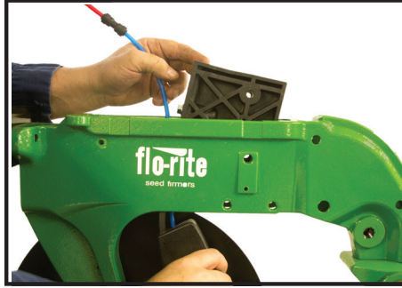
FIG. 2 MOUNT BLOCK
