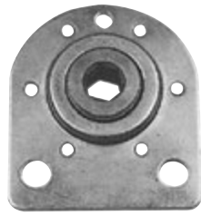
BEARING For clutch actuator shaft. 9/16" hex bore. Fits 7000 fle fold, 7200 & 1750. Replaces JD no. AA34259.
