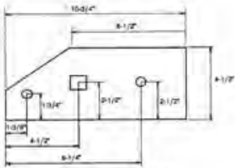
489465 RH LANDSIDE 542417 LH LANDSIDE 7/16 X 1-3/4 - 7/16 X 1-3/4
